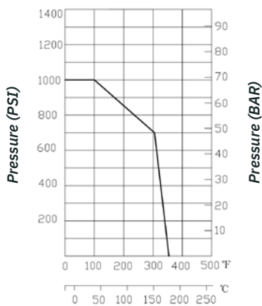
Pressure-Temp. Rating
