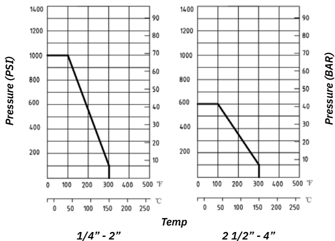
Pressure-Temp. Rating
