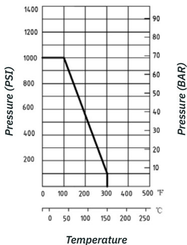
Pressure-Temp. Rating
